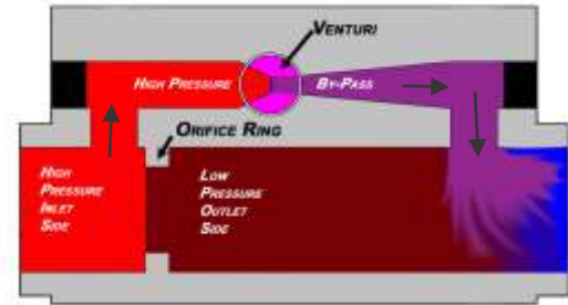
It's patented lateral-by-pass venturi permits the H 2 O Neutralizer to operate with no power...
