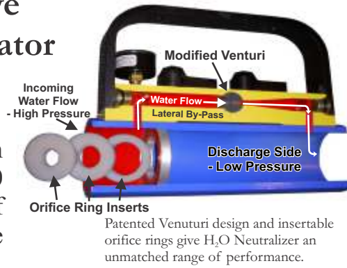
It's patented lateral-by-pass venturi permits the H 2 O Neutralizer to operate with no power...
